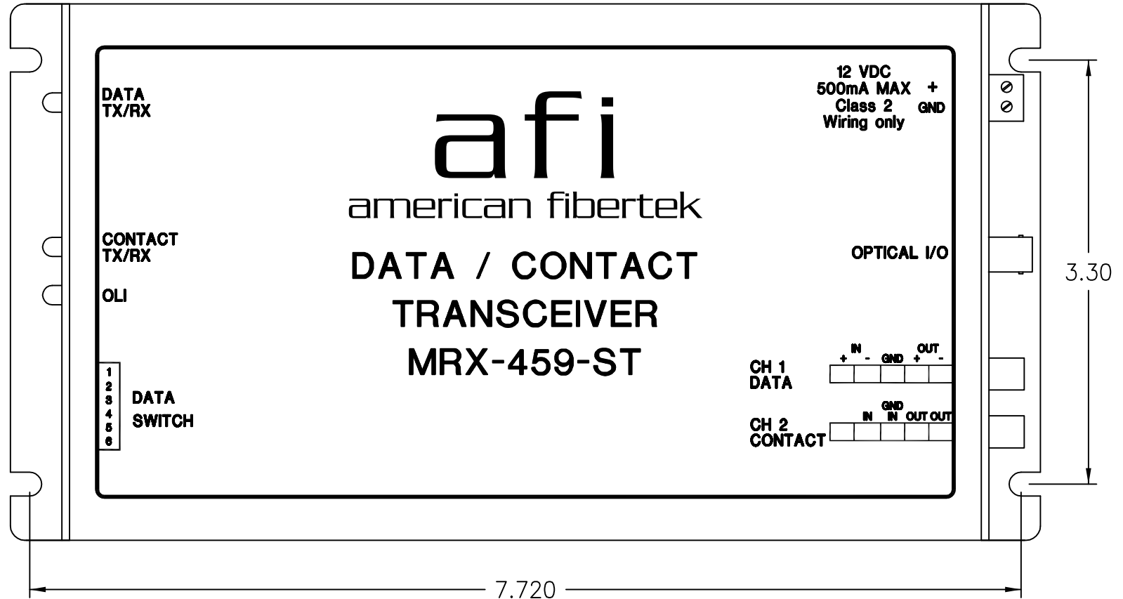
DATA CONNECTIONS
