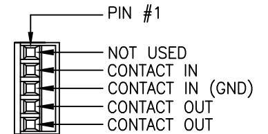
CONTACT CONNECTIONS
