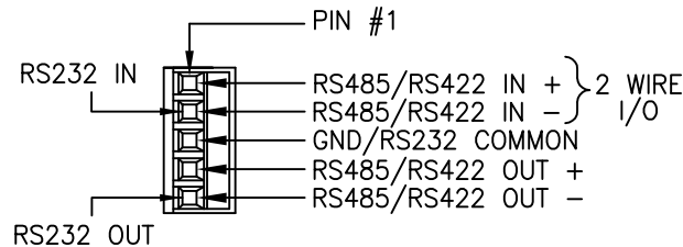
DATA CONNECTIONS
