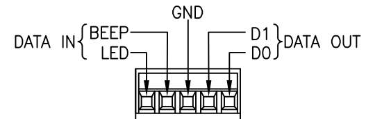
DATA CONNECTIONS
