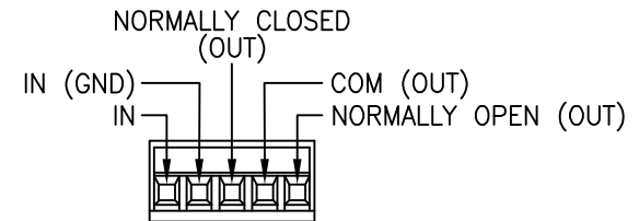
CONTACT CONNECTIONS
